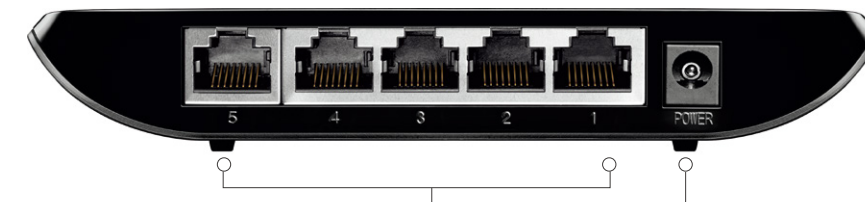
5 10/100/1000Mbps Ethernet Ports Power Socket
